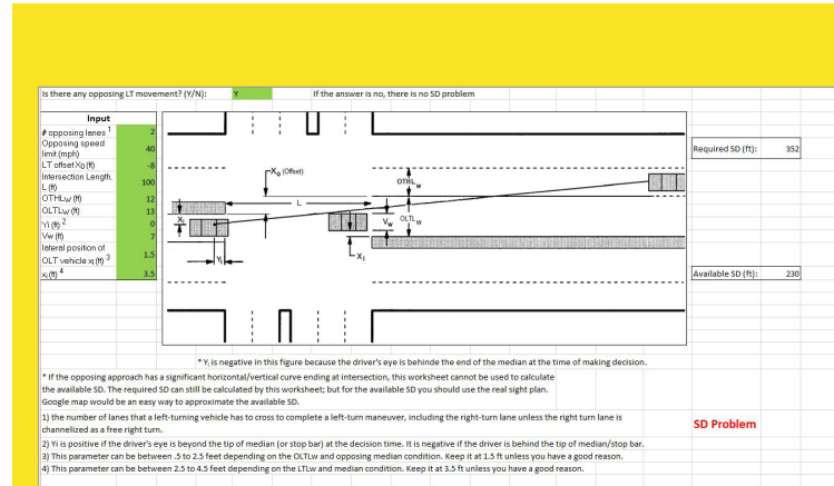
Screen Shot of Spreadsheet Tool
