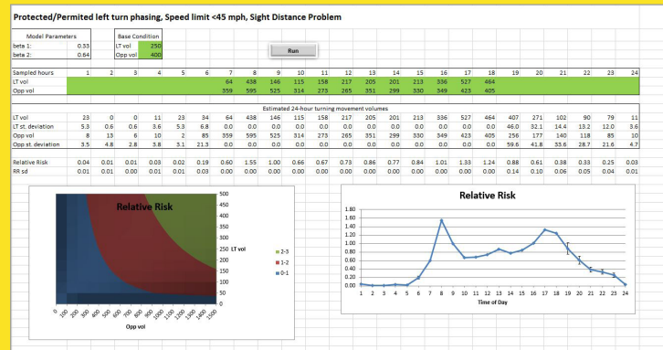
Screen Shot of Spreadsheet Tool
